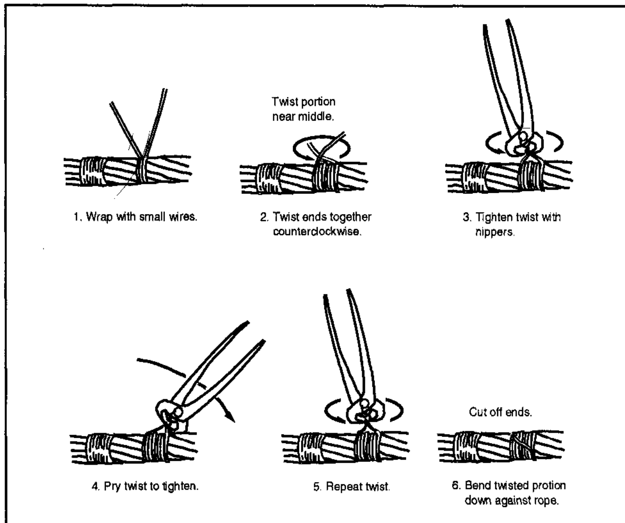
Figure 1-10. Seizing wire rope
