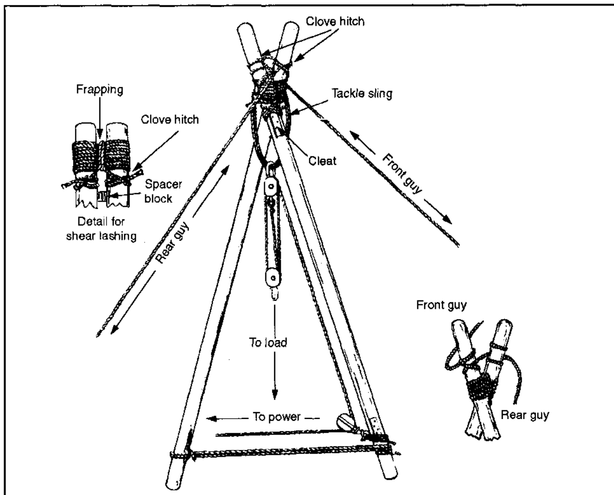
Figure 5-6. Lashing for shears
