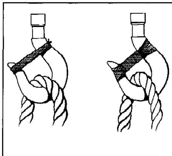
Figure 3-4. Mousing hooks
