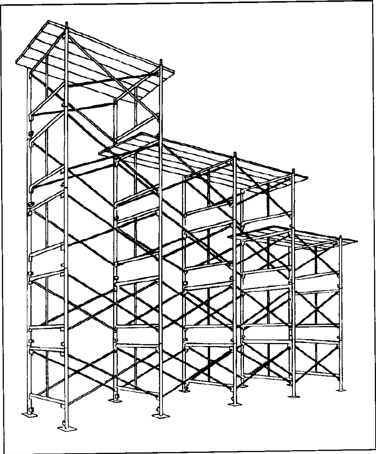
Figure 6-5. Independent scaffolding
