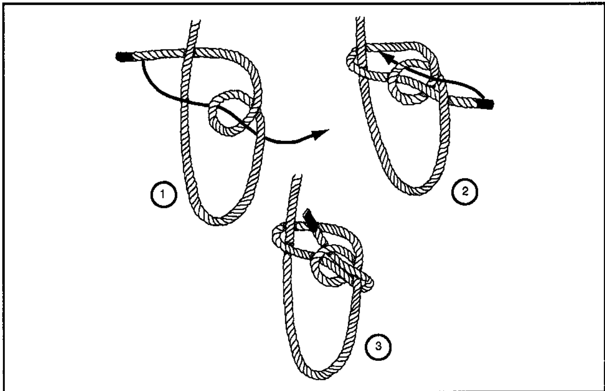
Figure 2-13. Running bowline
