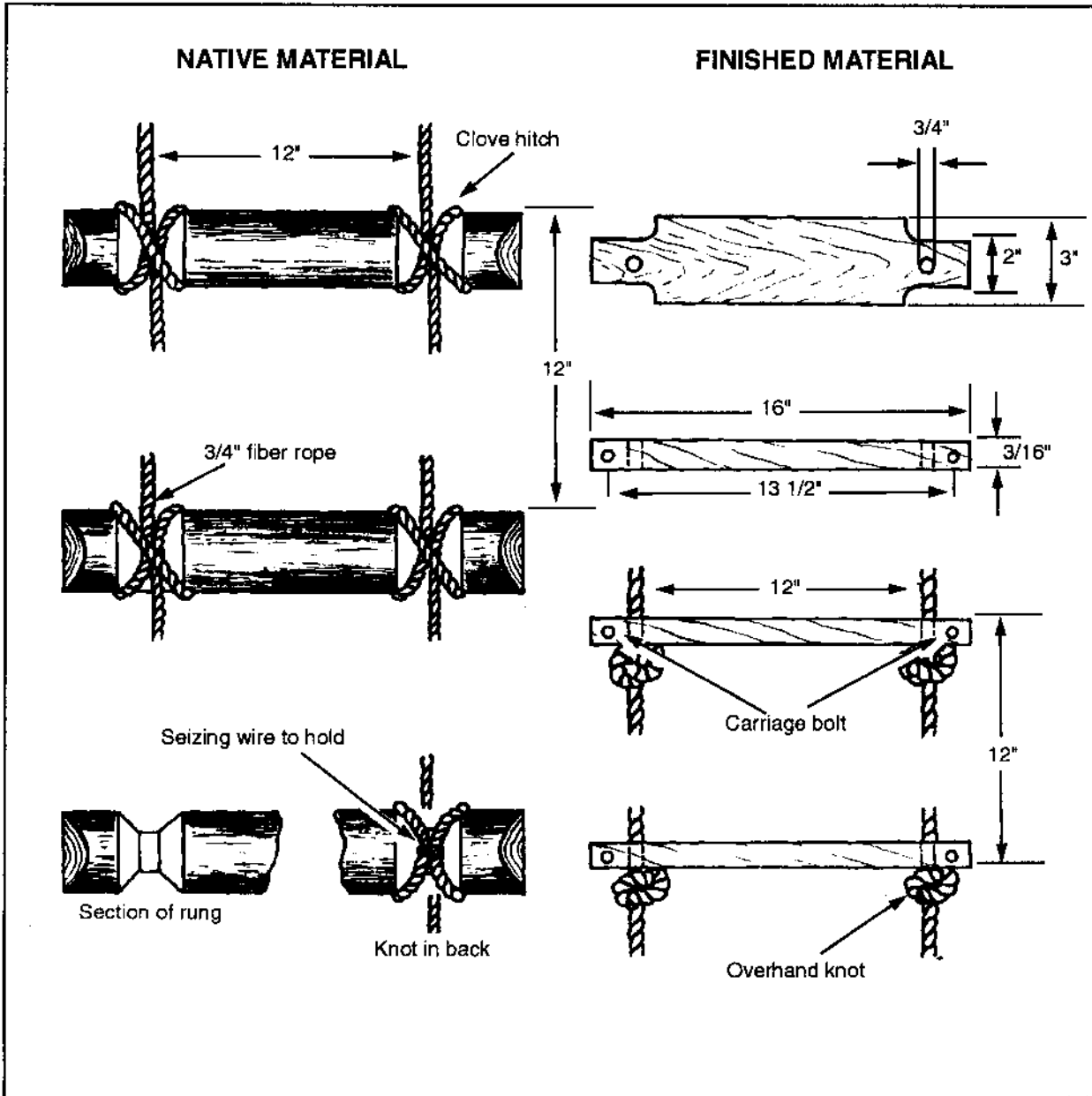
Figure 2-60. Wood rungs
