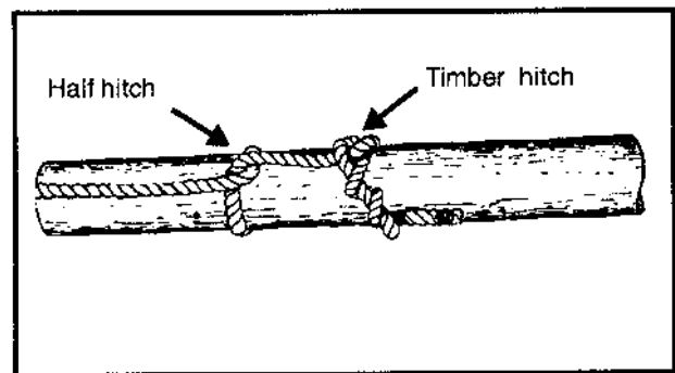
Figure 2-25. Timber hitch and half hitch
