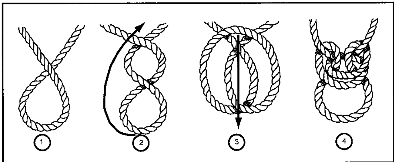
Figure 2-20. Butterfly knot
