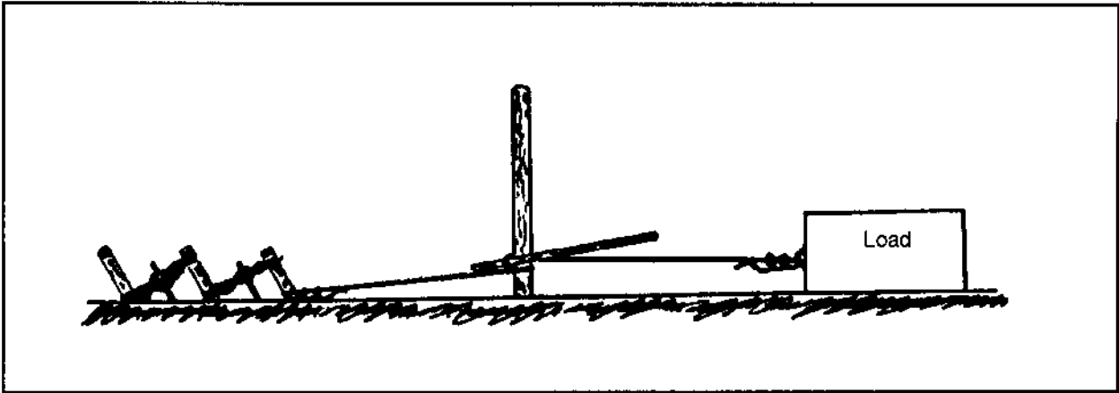
Figure 3-24. Spanish windlass
