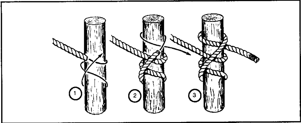
Figure 2-29. Mooring hitch
