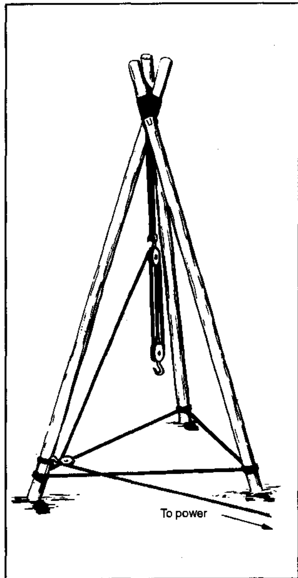
Figure 5-5. Assembled tripod
