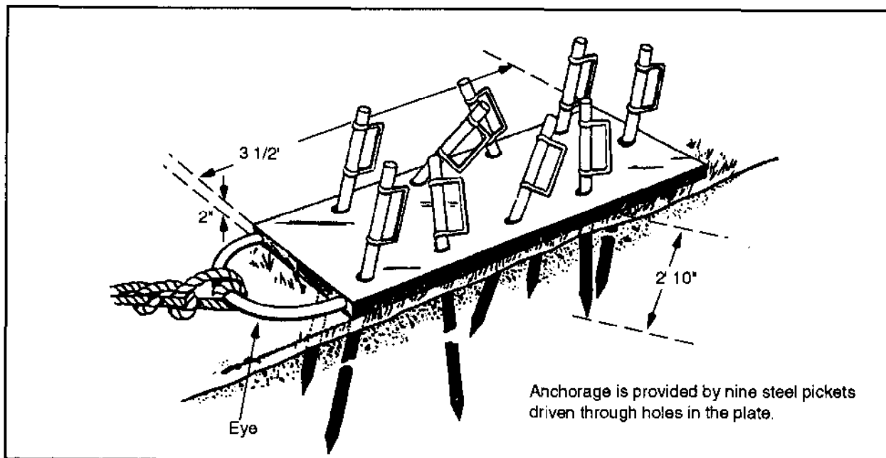
Figure 4-8. Standard steel-picket holdfast
