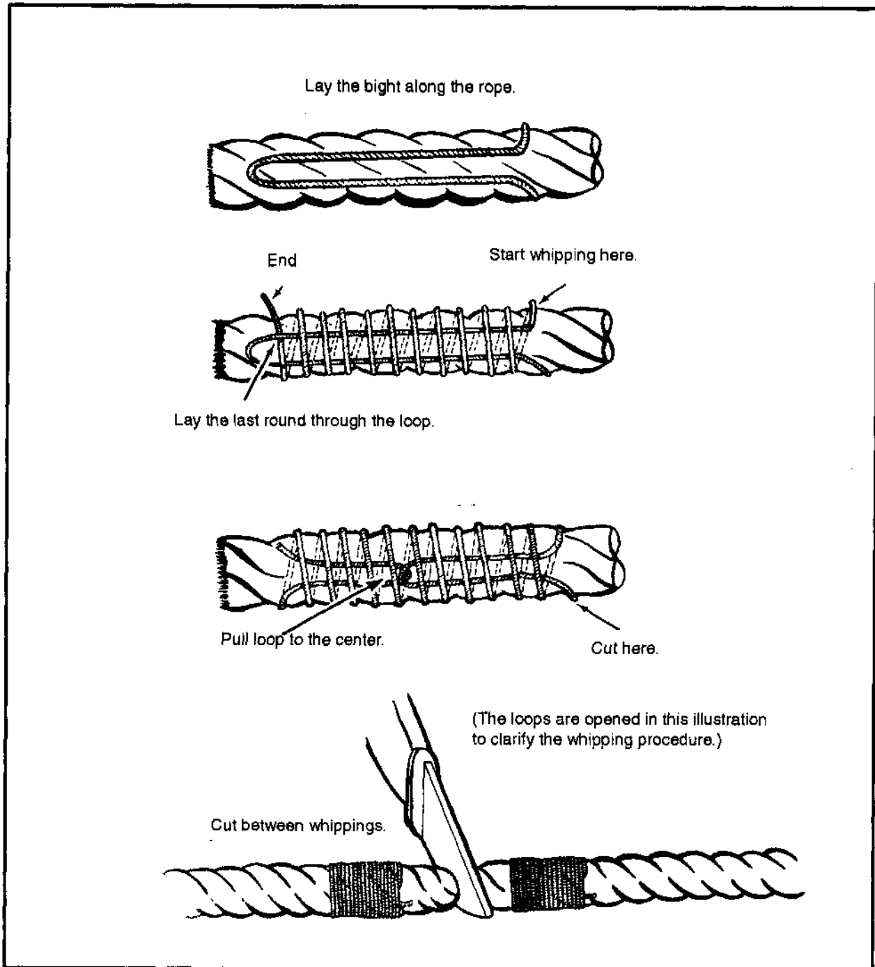
Figure 2-2. Whipping the end of a rope
