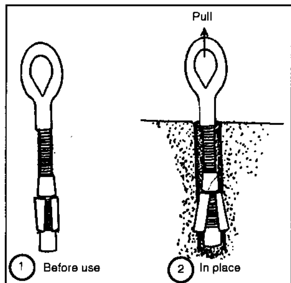
Figure 4-4. Rock anchor
